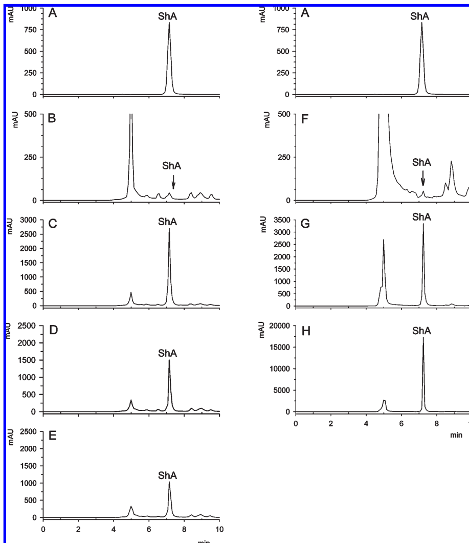
Figure 1. High-performance liquid chromatograms of shikimic acid standard solution (A), shikimic acid extracted from leaves of RS horseweed plants 0 (B), 3 (C), 7 (D), and 10 DAT (E), and shikimic acid extracted from leaves of S horseweed plants 0 (F), 3 (G), and 7 DAT (H). Each profile represents an equivalent amount of extract, normalized per 5 mg of tissue. ShA denotes shikimic acid. Please note the different scales of the y-axes.
